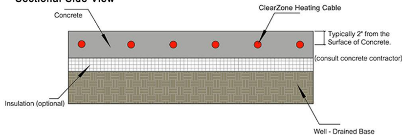
Illustration of ClearZone snow melting system in concrete.
